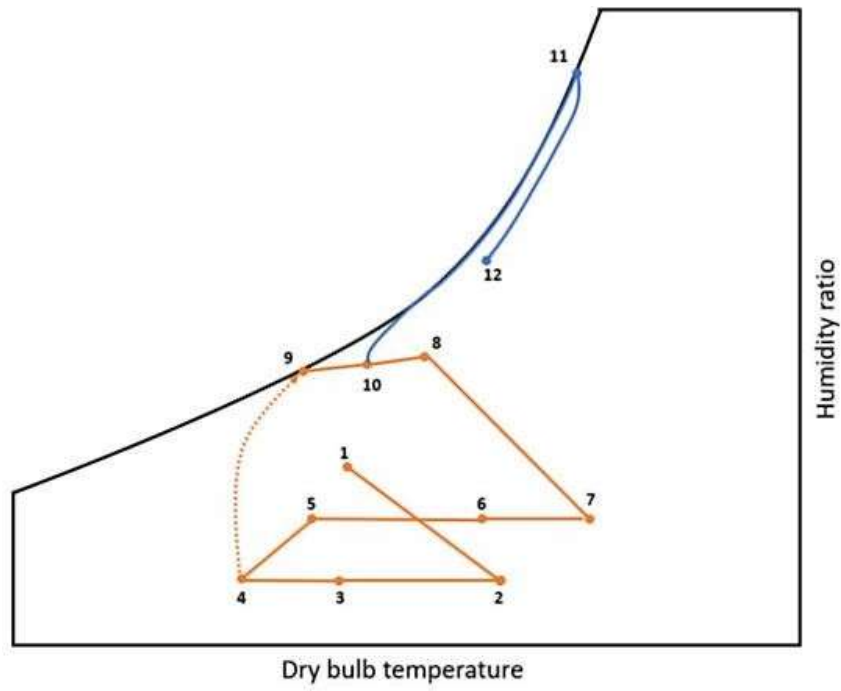
Figure2:Psychometricdiagramofthedesignprocess
